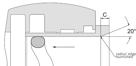
Cover by using a mounting sleeve
