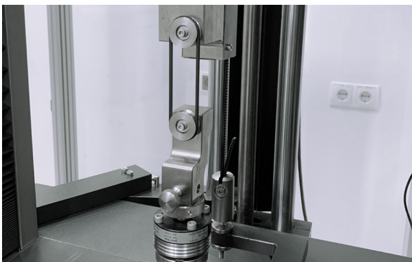
Tensile test on the final O-ring product
