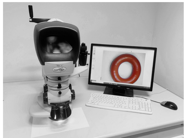
Surface inspection with a digital microscope
